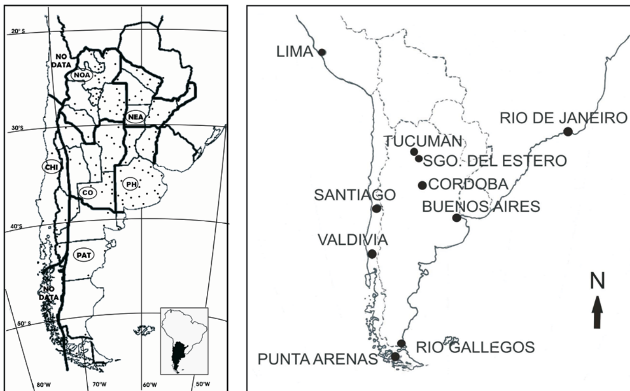
Figure 1 - Studied areas including the six sub-regions where the monthly and annual drought indices were calculated. The rain gauge stations are indicated (left). Likewise, the location of the geographic localities mentioned in this paper is shown (right).
